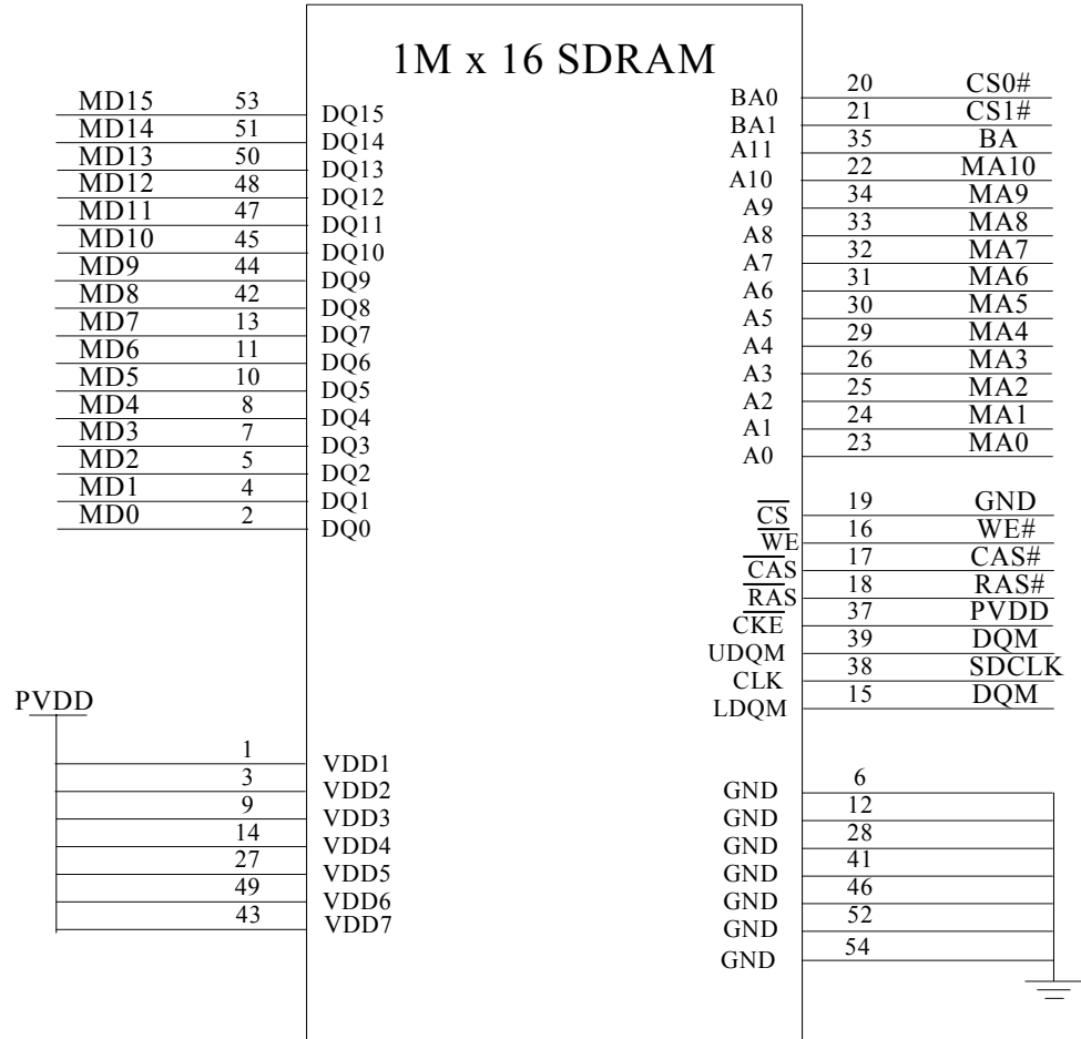
SDRAM_1MX16X4BANK CHIP
